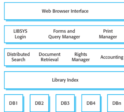
Figure: The architecture of the LIBSYS system.
